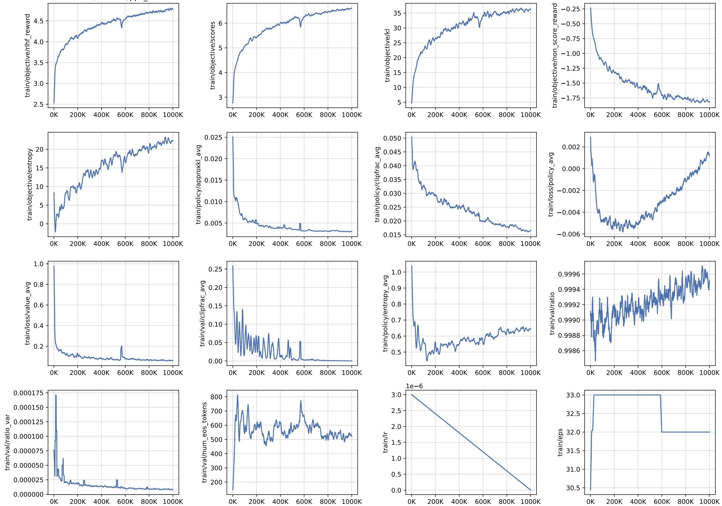
models/minimal/ppo_tldr
